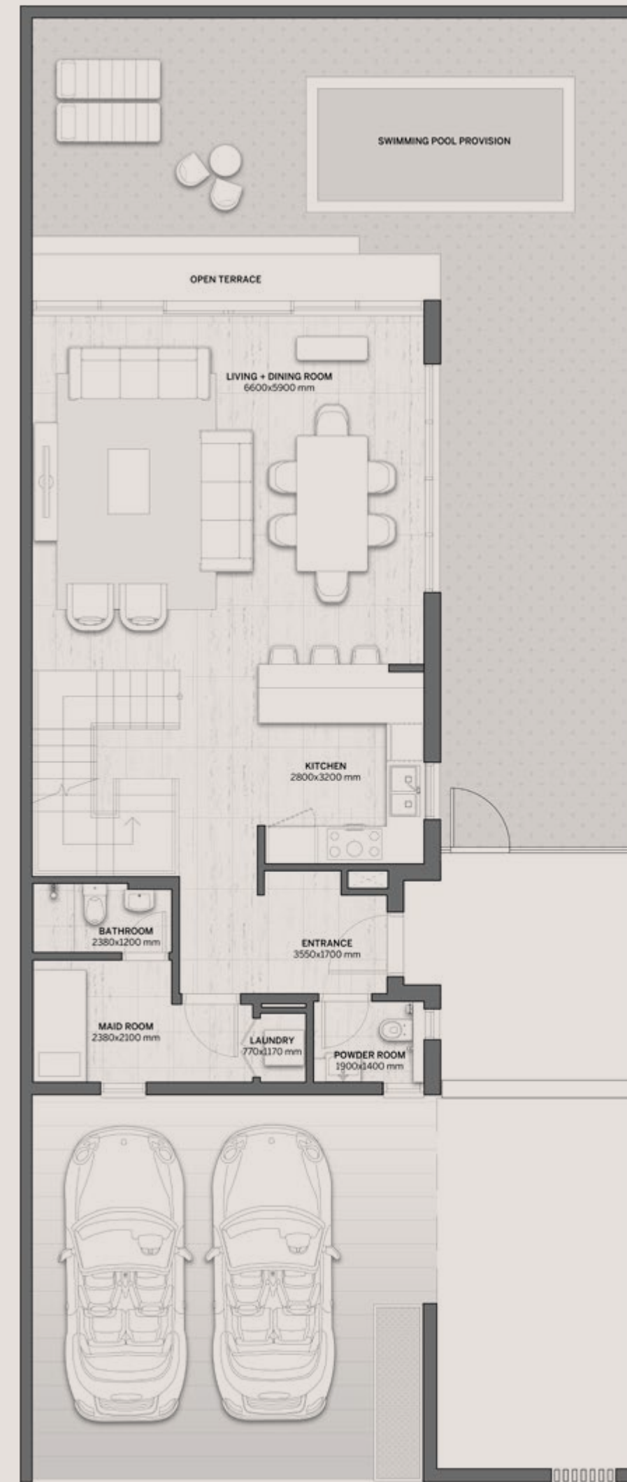
GROUND FLOOR
